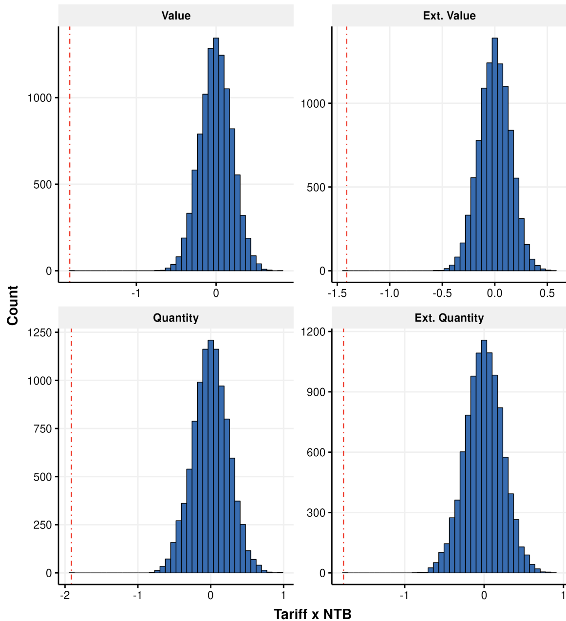
Figure B.4: Permutation test for the interaction coefficient, Tariff \times NTB , from Table 16. 10^4 permutations.
