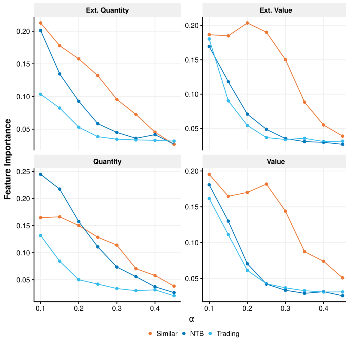
Figure D.3: Features importance for varying forest parameterization
